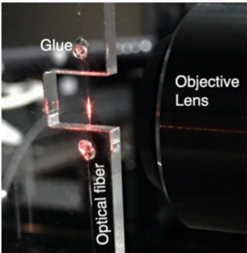
In-process measurement of micro/nano-fiber
