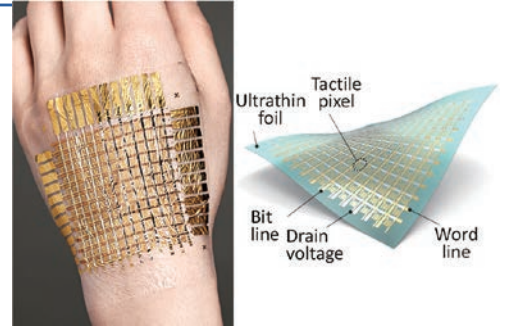
Touch sensors made with the world's lightest, thinnest and softest electronic circuits.
